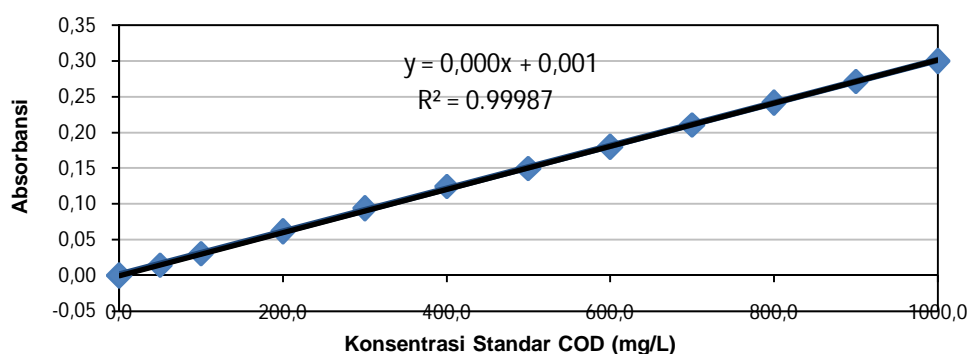
Gambar 3. Kurva kalibrasi larutan standar COD
